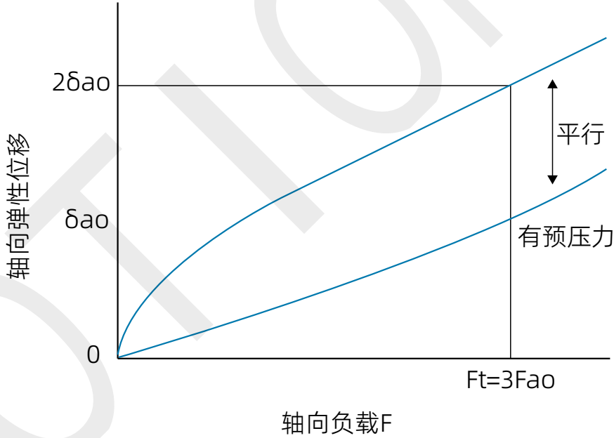
间隙规格和预压规格的弹性位移曲线
